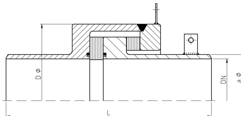
Insulating joint with connection for ex-proof spark gaps.
