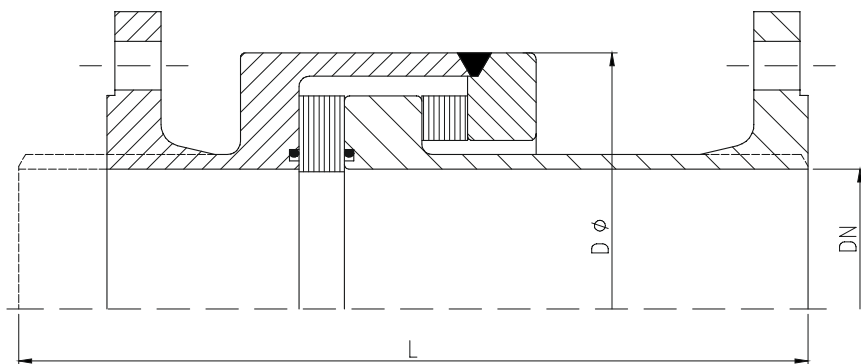
Insulating joint with flange connection on one or both sides.
